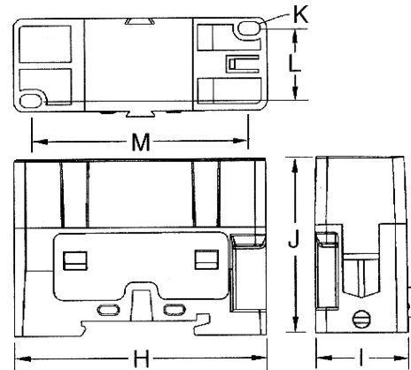
100 amp holder
