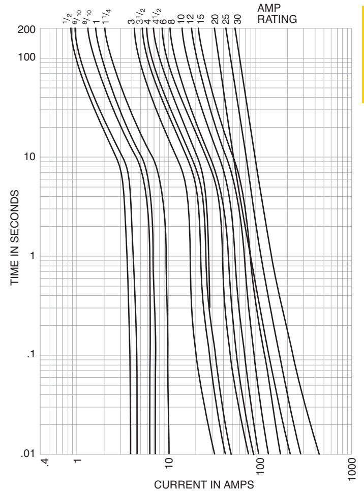
Time-current characteristics — average melt
