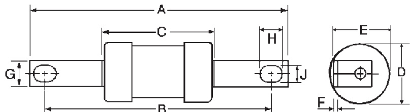
Dimensional Data
